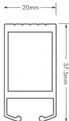
Track HT6000 Profile
