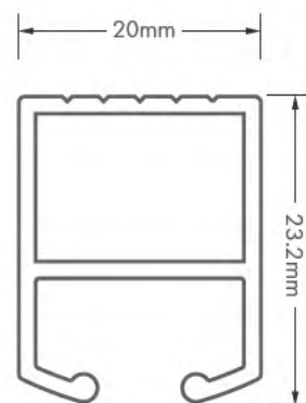
Track MT6000 Profile
